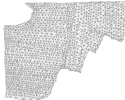
TIN surface in AutoCAD
